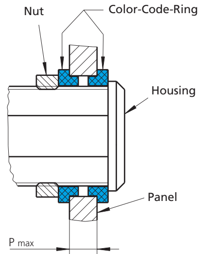
Mounting Example:
