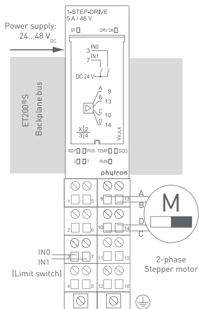
Connection diagram
