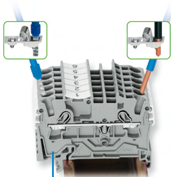
• Bornes sur rail Rail-Mounted Terminal Blocks TOPJOB® S Series
